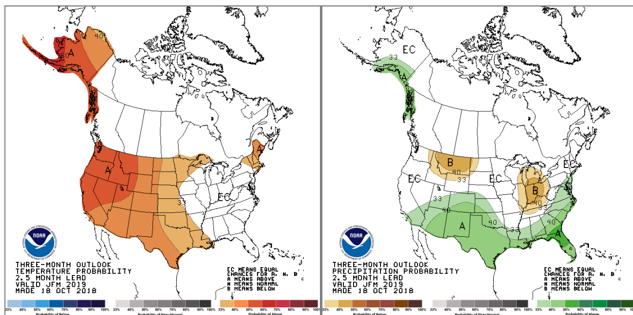
Figure 18. Three-month temperature (left) and precipitation (right) outlook for Jan-Mar 2019.
